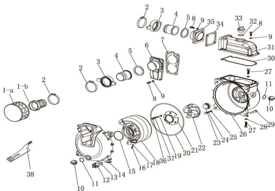
Detailed list of parts for 3" trash pump: (Model:PTR80H)
