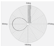
G-8 2.4 GHz antenna vertical plane pattern
