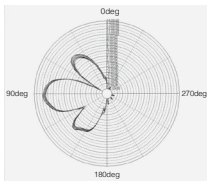
G-8 5.8 GHz antenna vertical plane pattern
