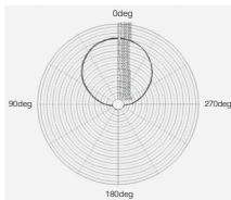
G-8 2.4 GHz antenna azimuth plane pattern
