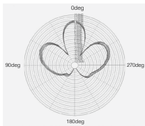
G-8 5.8 GHz antenna azimuth plane pattern
